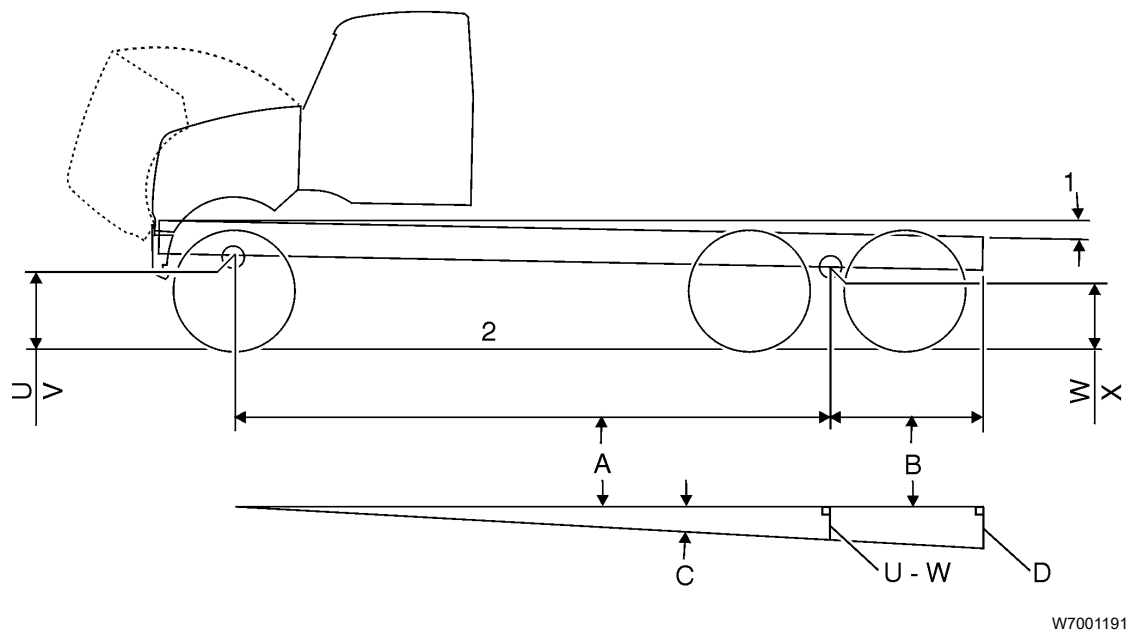
Negative Frame Rake
