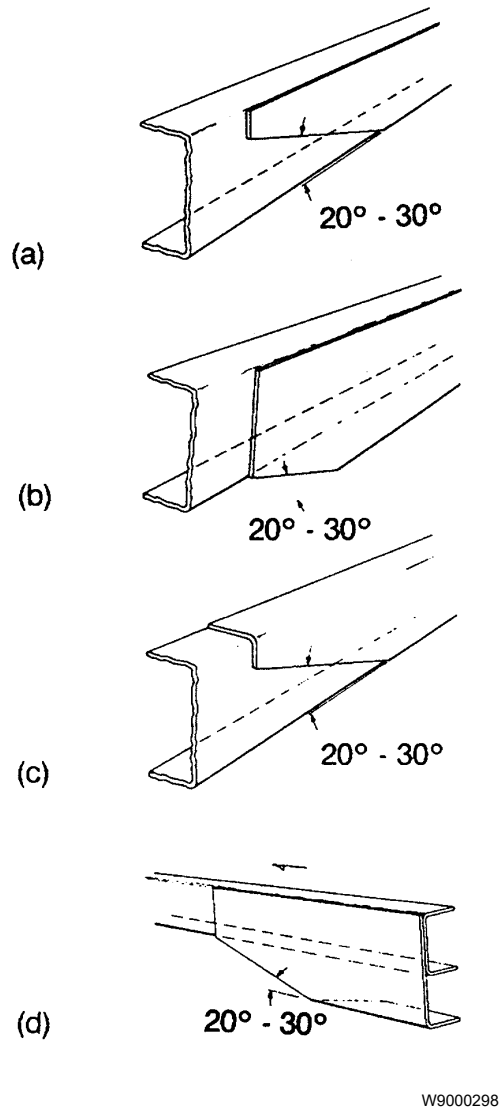
Fig. 6 End Tapering, Fish Plates with 'L' Reinforcements
