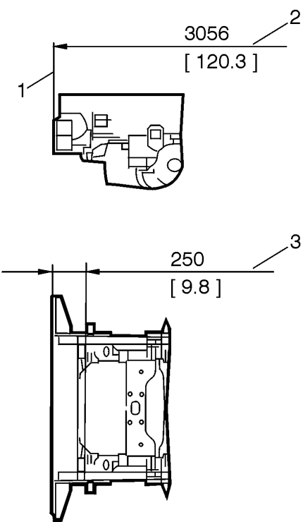
View A: HD Front Closing Crossmember with 8 in Frame Extension
