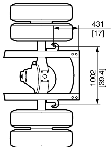
Tow Hooks, Tapered Rear Frame End
