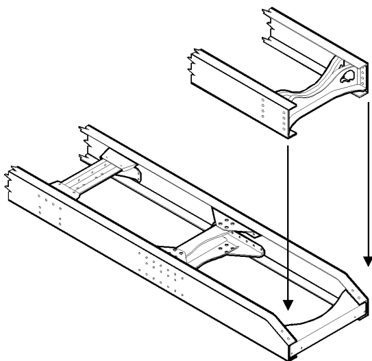
Closing Crossmember
