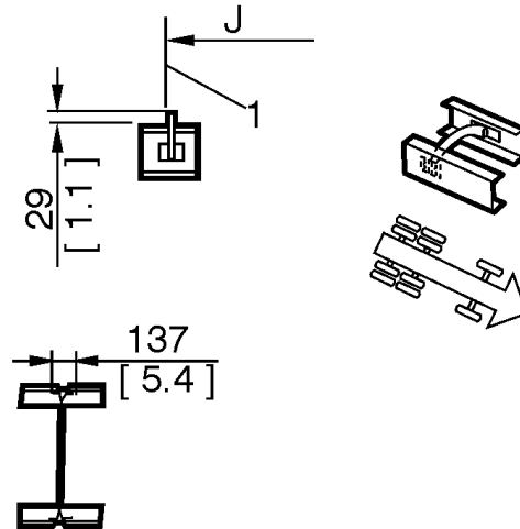
View C: Optional Crossmembers
