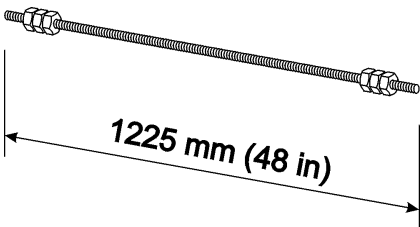
Threaded rods
