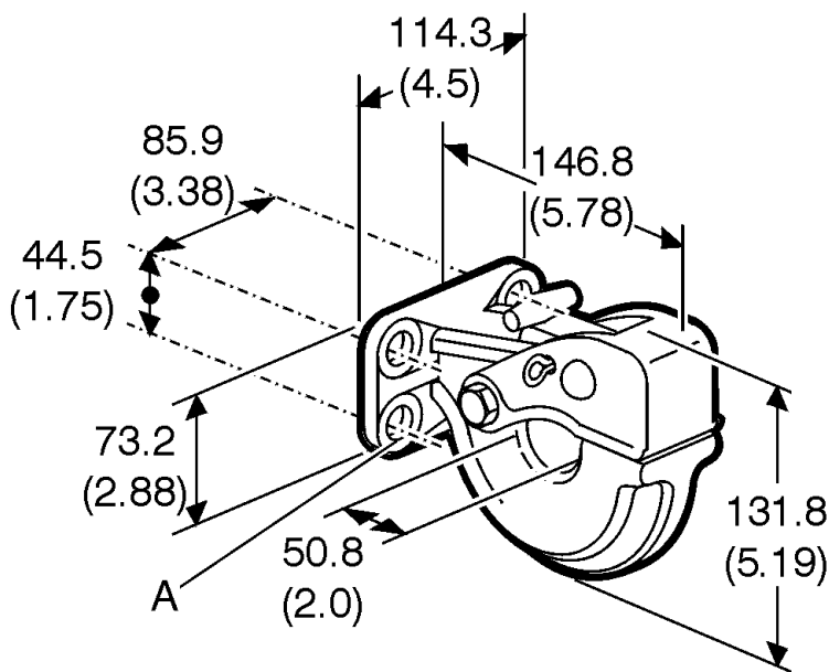
PH-5 Rigid Pintle Hook
